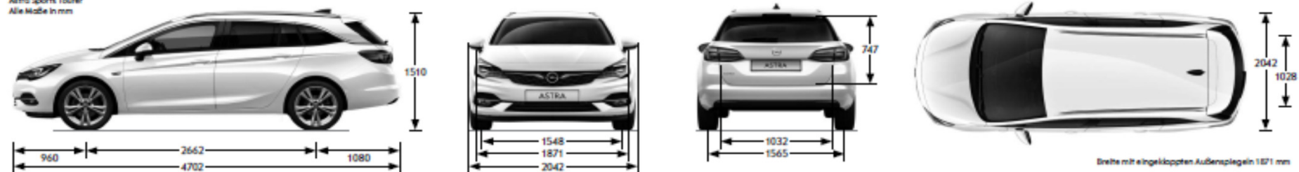
Astra Sports Tourer Alle Maße in mm
